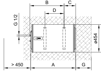
Fig. 2: Horizontal installation on a wall
