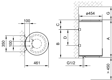
Fig. 1: Vertical installation on a wall
